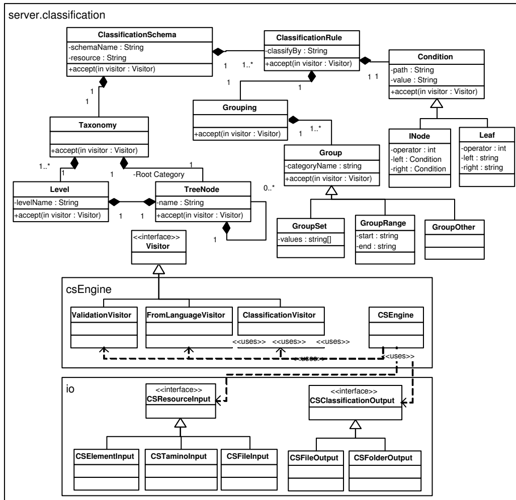
Fig. 10. Design of the Classification Module
