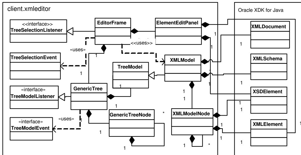
Fig. 8. Class Diagram of the XML Editor
