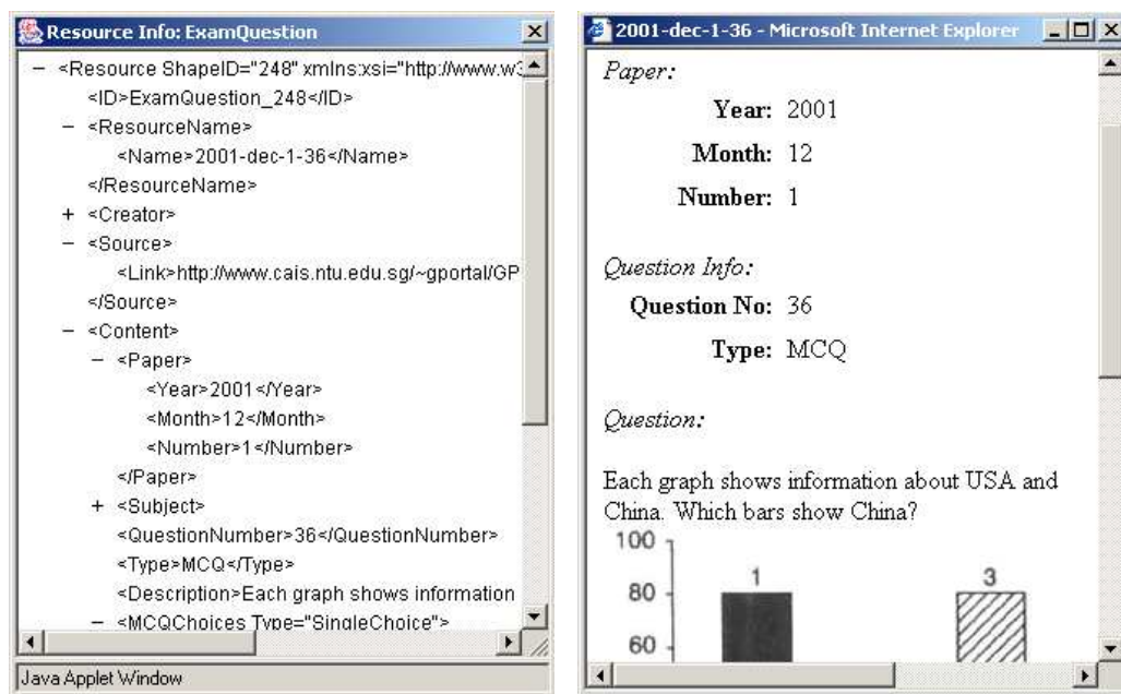
(a) Raw XML Content
