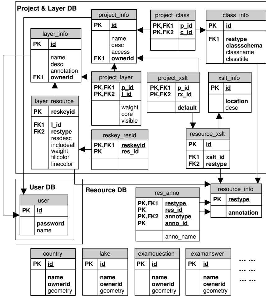
Fig. 6. Database Schema Design in the Informix RDBMS
