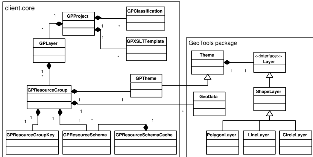
Fig. 5. Class Diagram of Client Side Resource Representation
