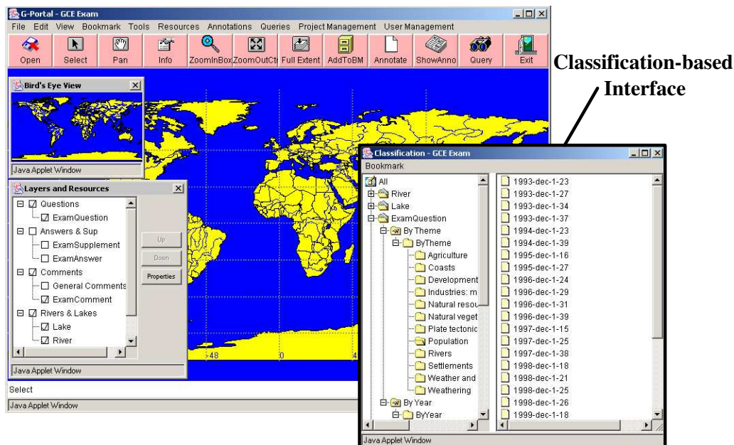
Fig. 1. Map-based and Classification-based Interfaces
