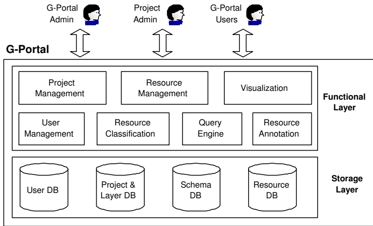
Fig. 3. Design Architecture of G-Portal
